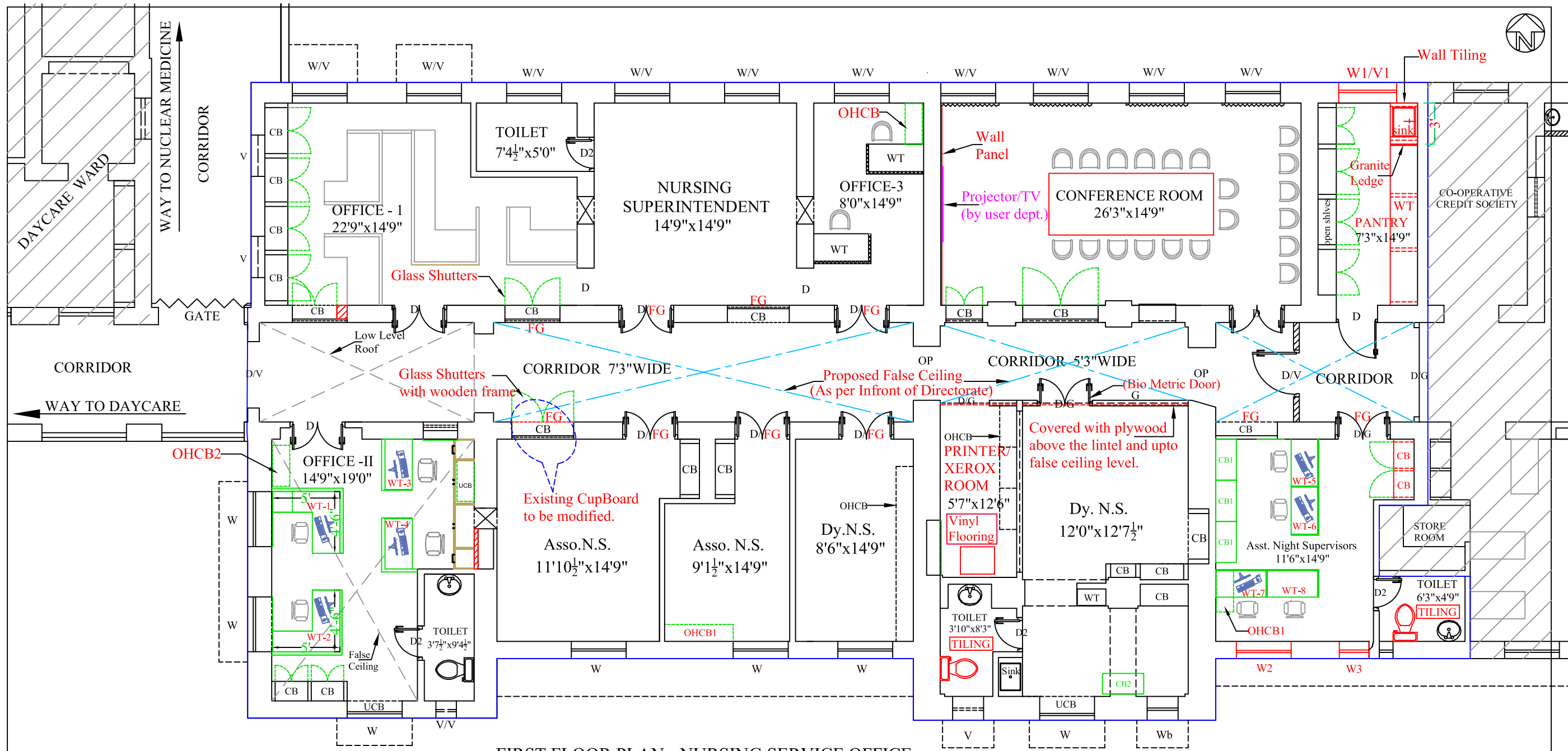
FIRST FLOOR PLAN - NURSING SERVICE OFFICE
